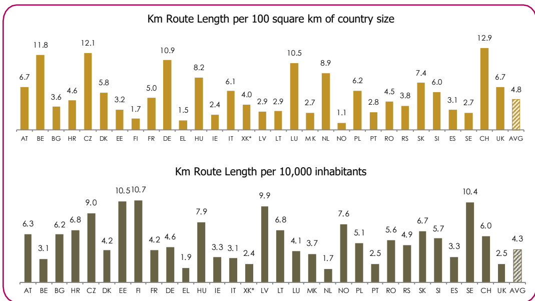
Figure 3 – Network density with respect to country area and population in 2022
